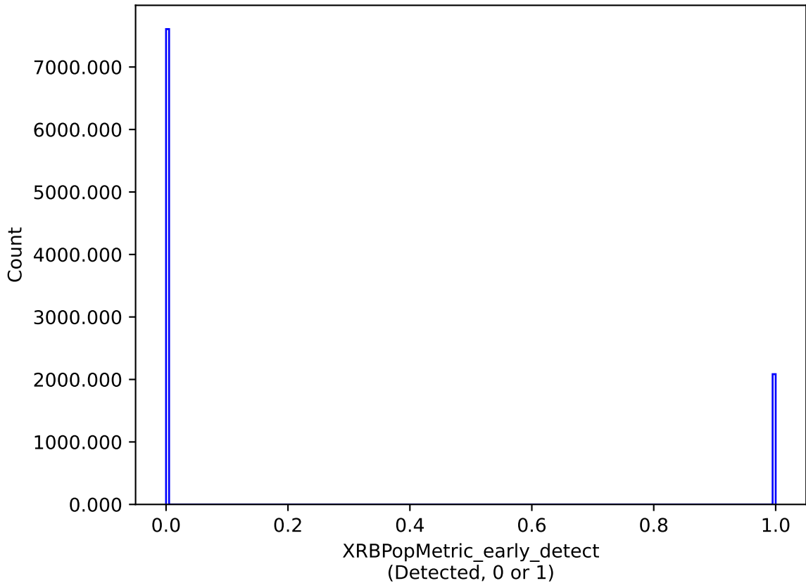
internal_u_expt38_nscale1.2v3.4_10yrs : XRBPoMetric_early_detect
