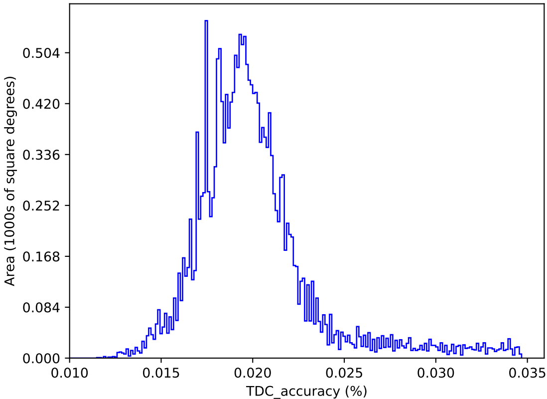
internal_u_expt38_nscale1.2v3.4_10yrs : TDC_accuracy
