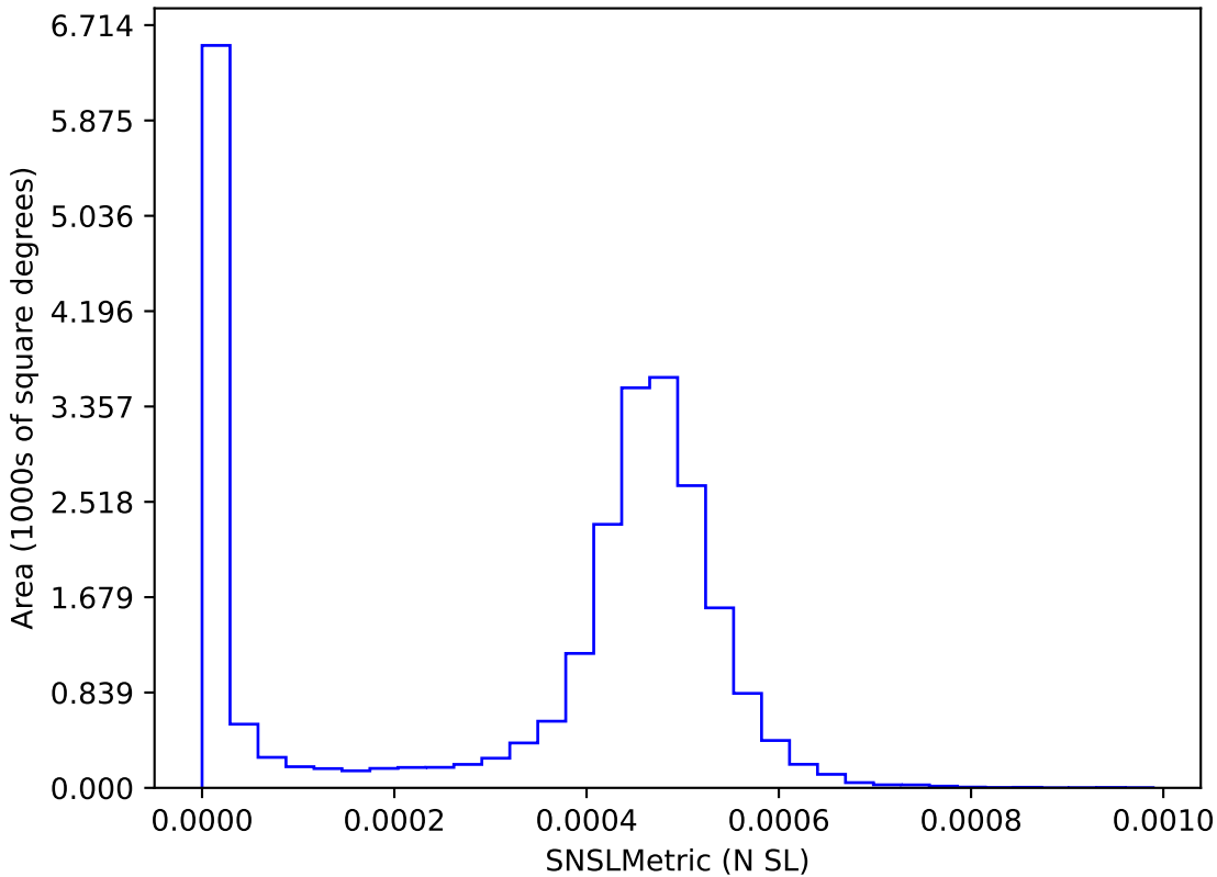
internal_u_expt38_nscale1.2v3.4_10yrs : SNSLMetric
