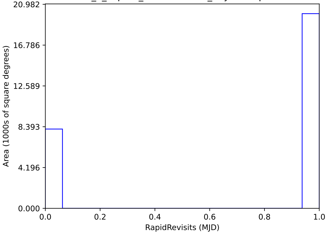
internal_u_expt38_nscale1.2v3.4_10yrs : RapidRevisits
