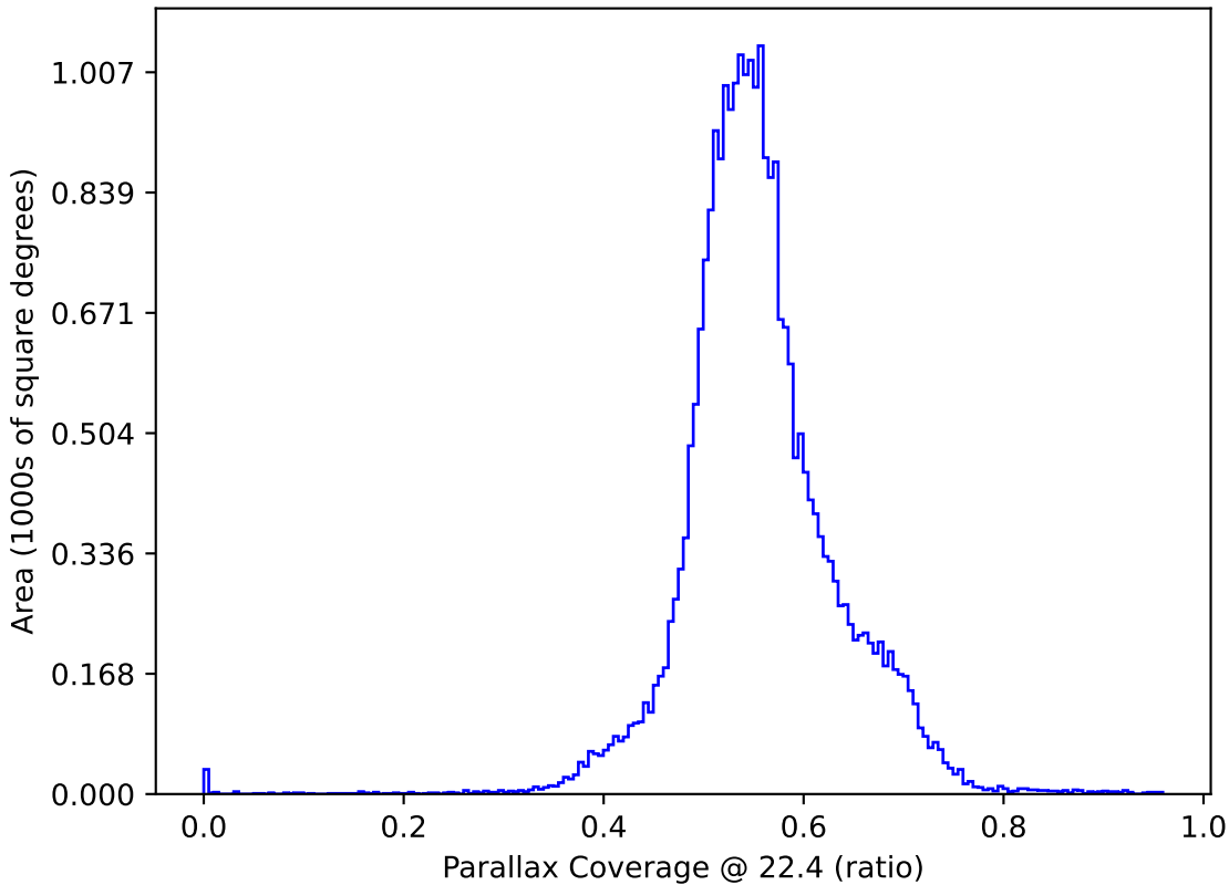
internal_u_expt38_nscale1.2v3.4_10yrs : Parallax Coverage @ 22.4
