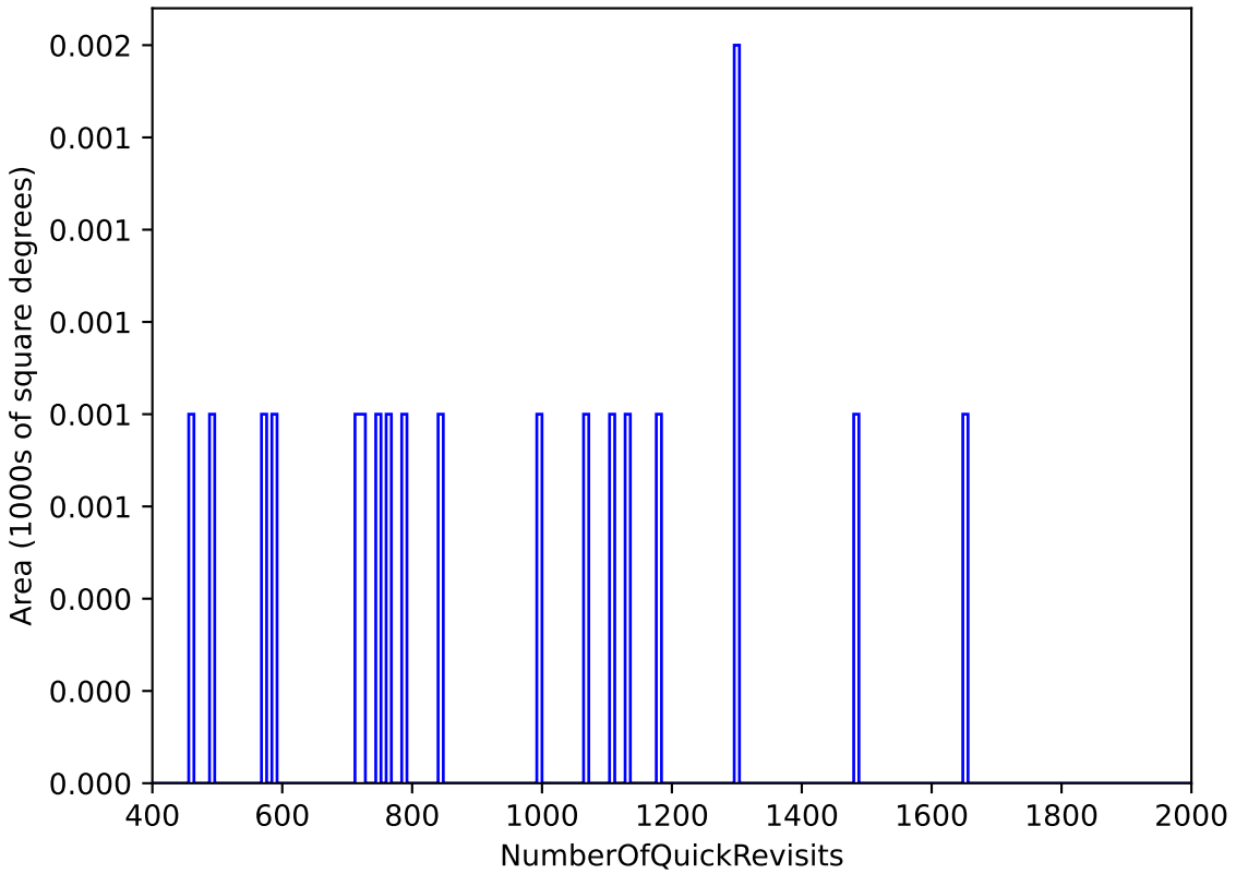
internal_u_expt38_nscale1.2v3.4_10yrs : NumberOfQuickRevisits
