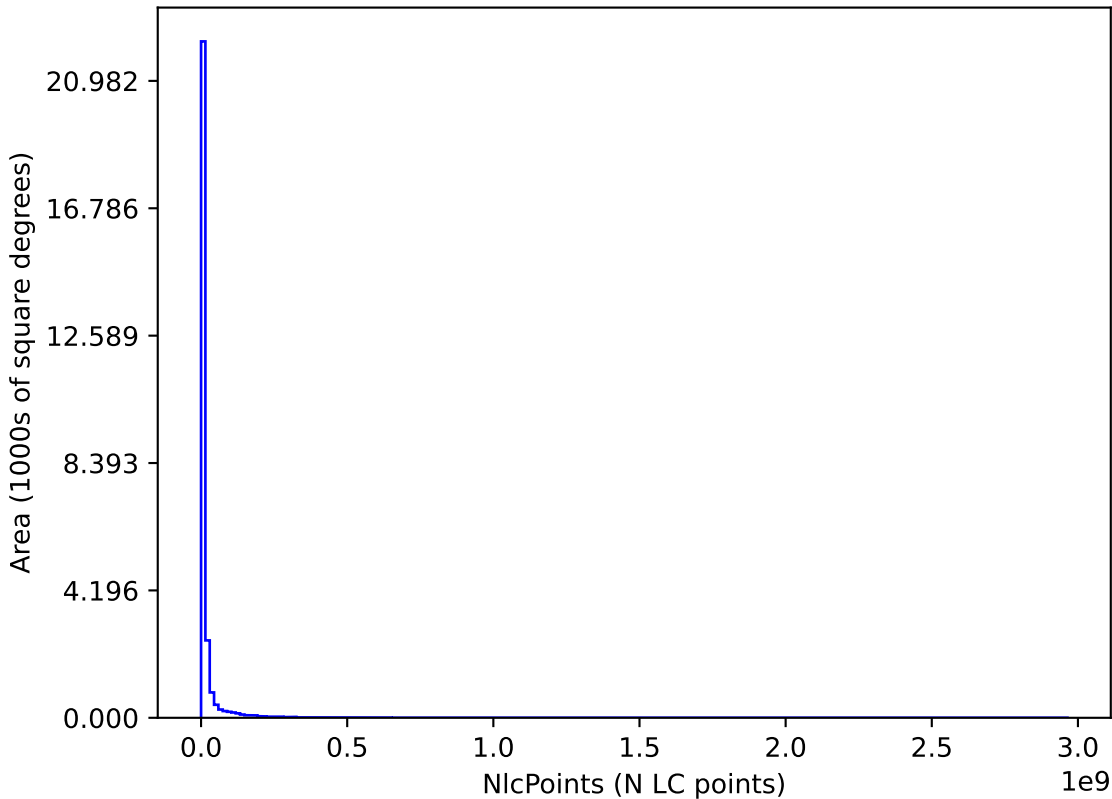
internal_u_expt38_nscale1.2v3.4_10yrs : NlcPoints
