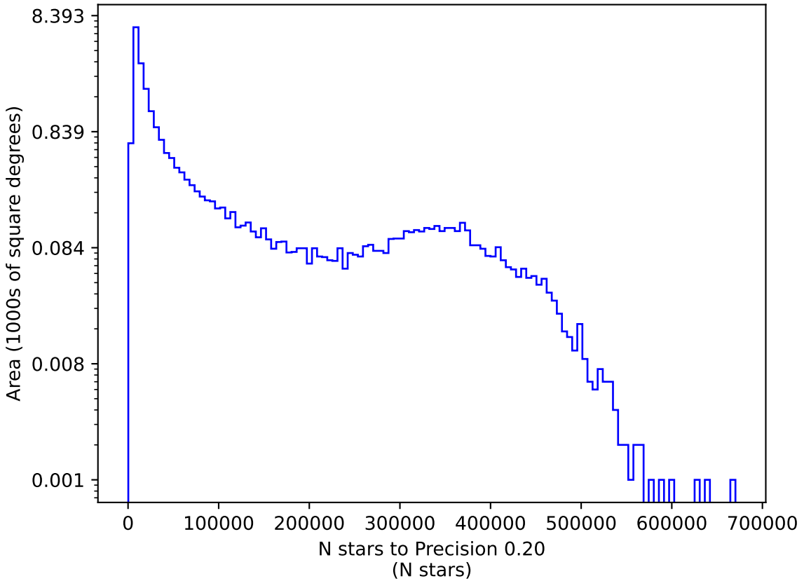
internal_u_expt38_nscale1.2v3.4_10yrs y: N stars to Precision 0.20
