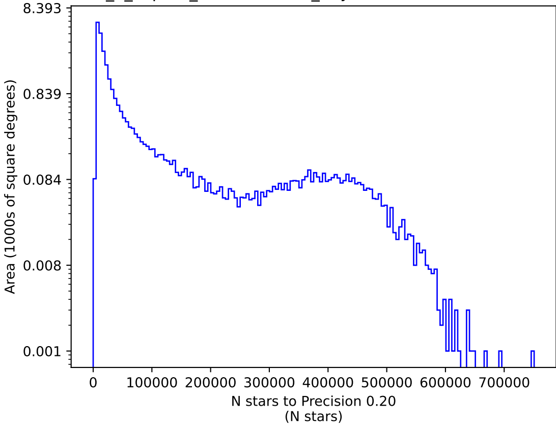
internal_u_expt38_nscale1.2v3.4_10yrs i: N stars to Precision 0.20
