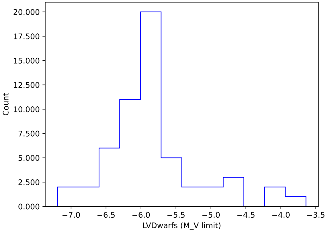
internal_u_expt38_nscale1.2v3.4_10yrs gi: LVDwarfs
