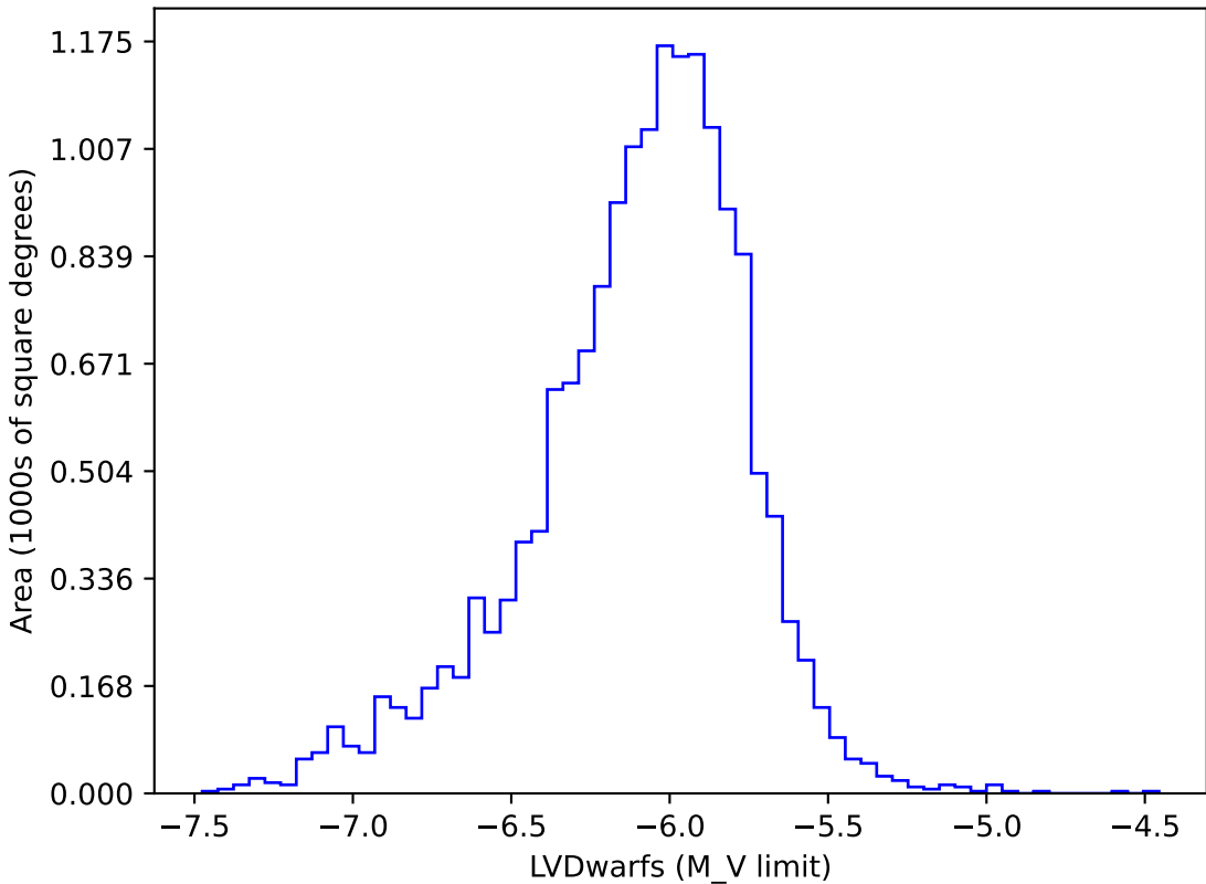
internal_u_expt38_nscale1.2v3.4_10yrs gi: LVDwarfs
