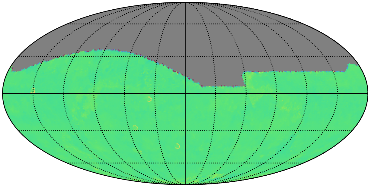
internal_u_expt38_nscale1.2v3.4_10yrs r: Kuiper rotTelPos
