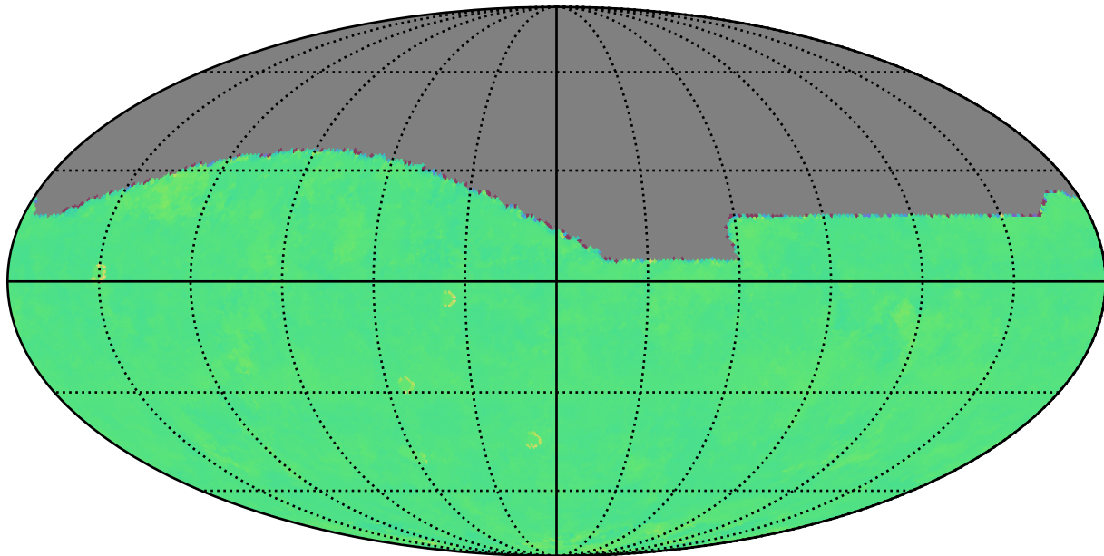
internal_u_expt38_nscale1.2v3.4_10yrs i: Kuiper rotTelPos
