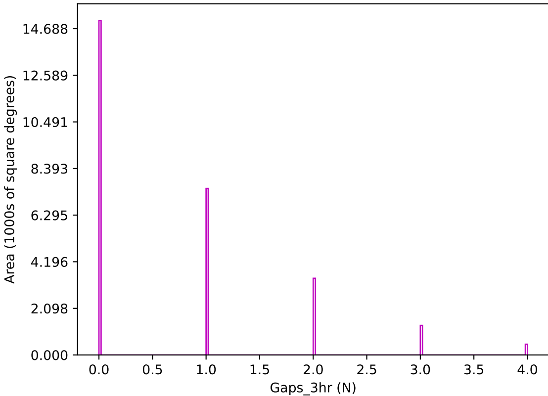
internal_u_expt38_nscale1.2v3.4_10yrs z band: Gaps_3hr
