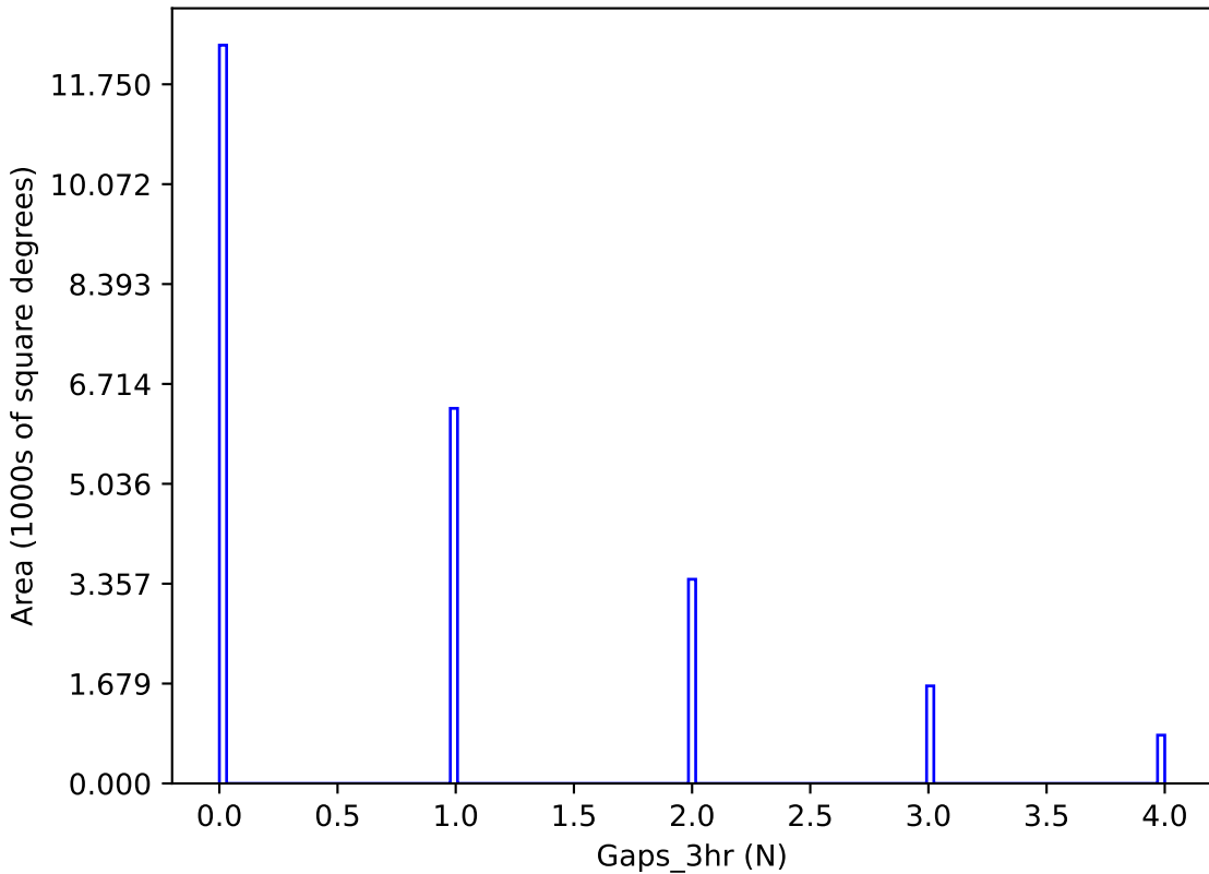
internal_u_expt38_nscale1.2v3.4_10yrs y band: Gaps_3hr
