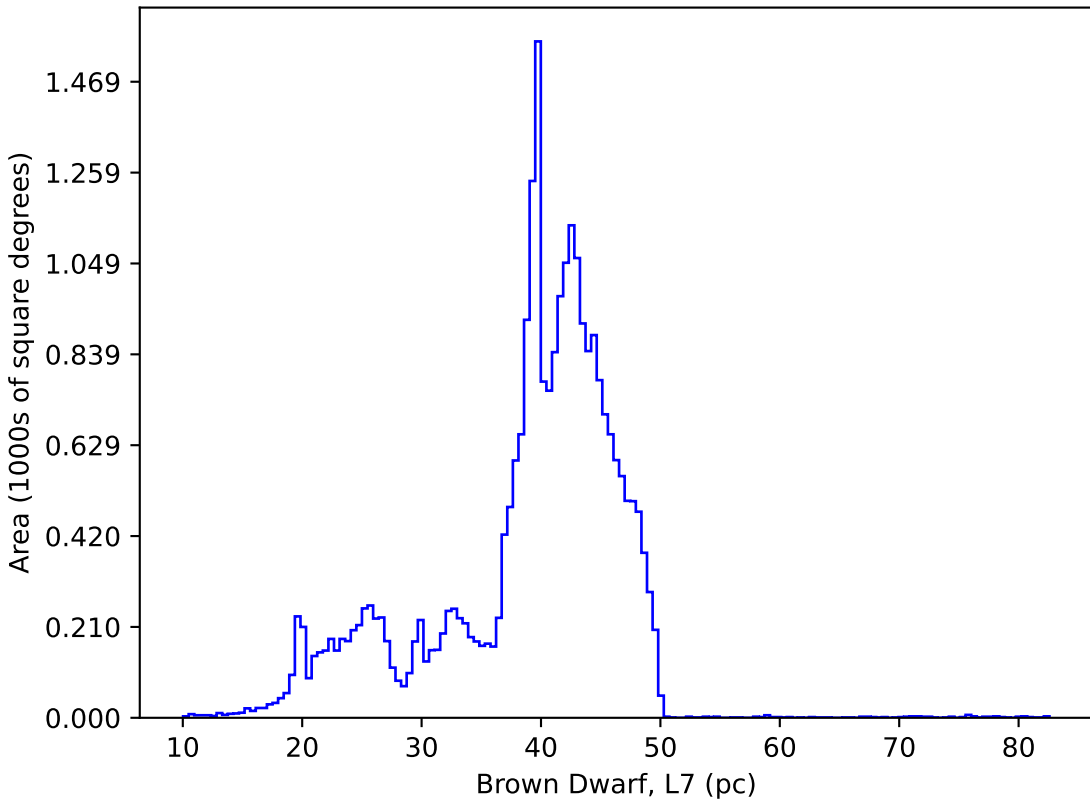
internal_u_expt38_nscale1.2v3.4_10yrs : Brown Dwarf, L7
