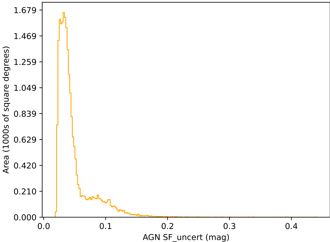
internal_u_expt38_nscale1.2v3.4_10yrs r band: AGN SF_uncert
