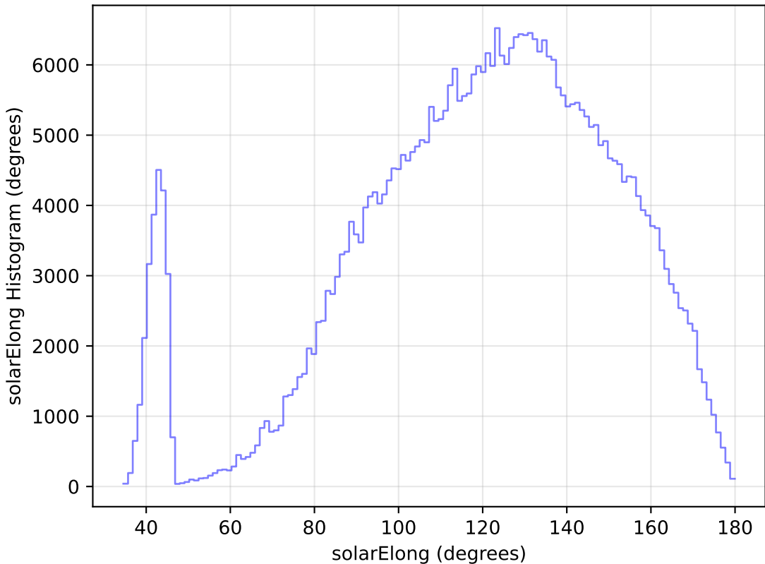
internal_u_expt38_nscale1.2v3.4_10yrs WFD z band: solarElong Histogram
