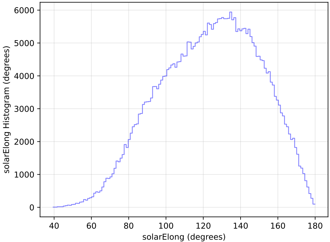
internal_u_expt38_nscale1.2v3.4_10yrs WFD y band: solarElong Histogram
