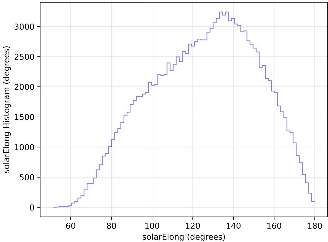
internal_u_expt38_nscale1.2v3.4_10yrs WFD u band: solarElong Histogram
