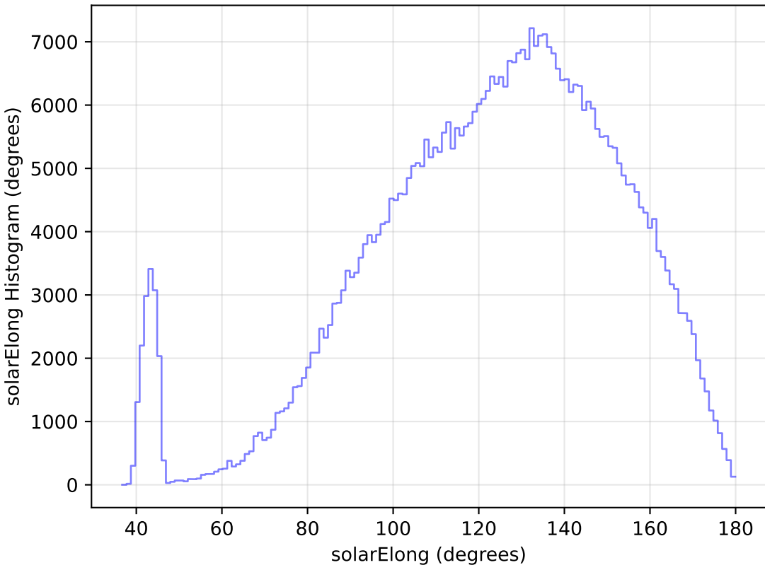
internal_u_expt38_nscale1.2v3.4_10yrs WFD r band: solarElong Histogram
