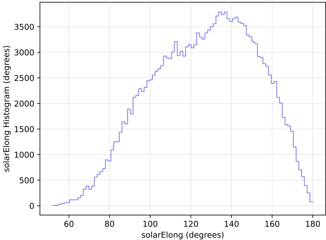
internal_u_expt38_nscale1.2v3.4_10yrs WFD g band: solarElong Histogram
