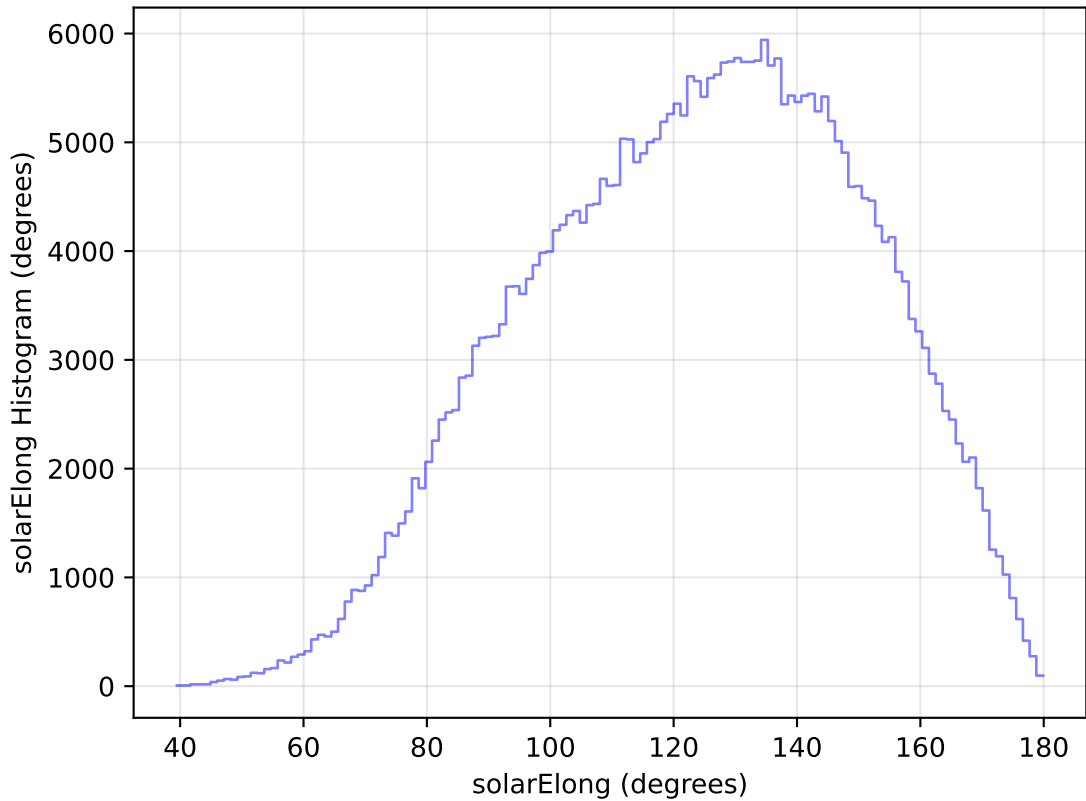
internal_u_expt38_nscale1.2v3.4_10yrs All sky y band: solarElong Histogram
