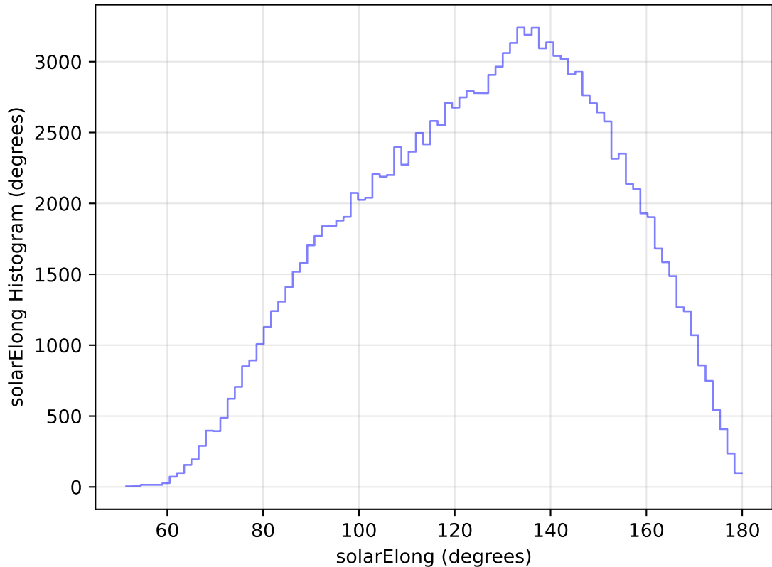
internal_u_expt38_nscale1.2v3.4_10yrs All sky u band: solarElong Histogram
