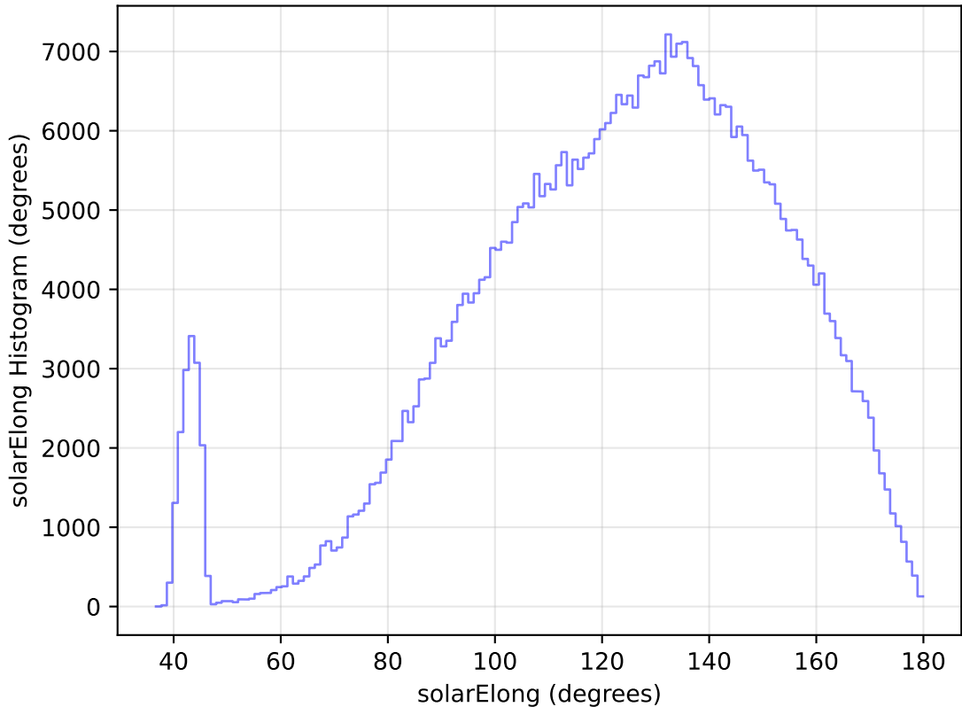
internal_u_expt38_nscale1.2v3.4_10yrs All sky r band: solarElong Histogram
