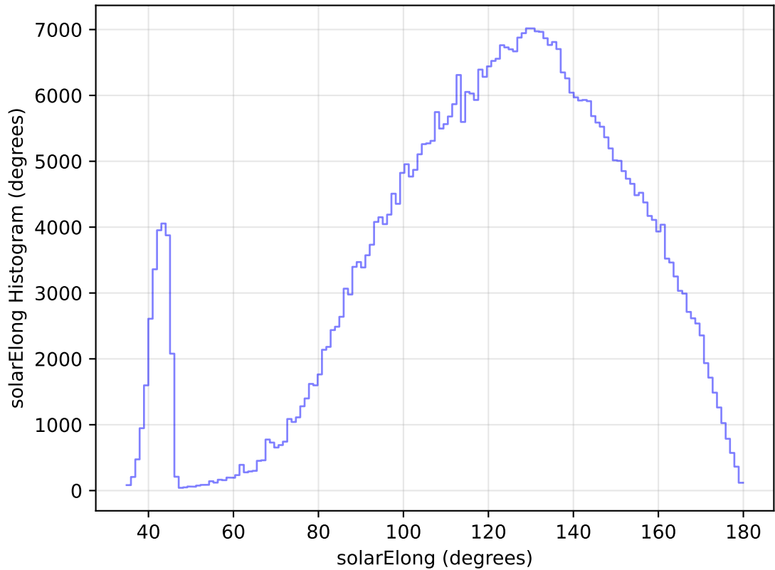
internal_u_expt38_nscale1.2v3.4_10yrs All sky i band: solarElong Histogram
