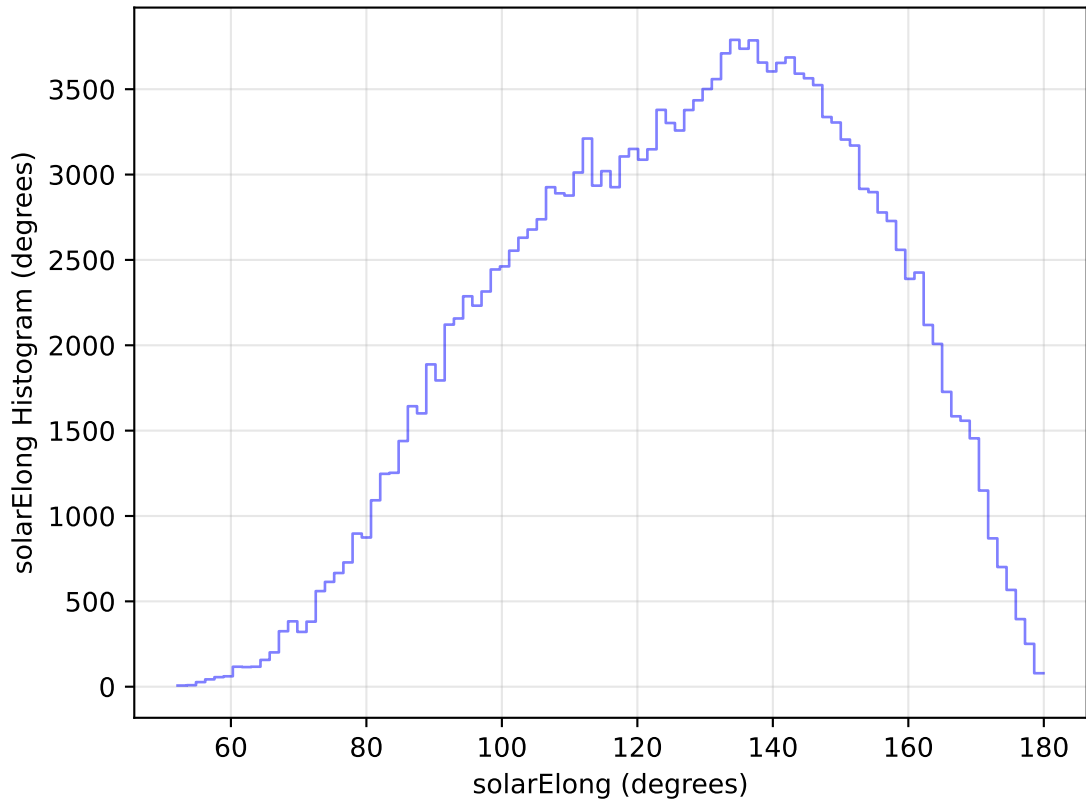
internal_u_expt38_nscale1.2v3.4_10yrs All sky g band: solarElong Histogram
