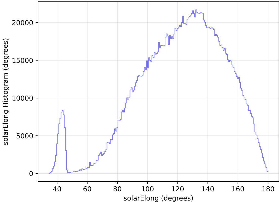
internal_u_expt38_nscale1.2v3.4_10yrs All sky all bands: solarElong Histogram
