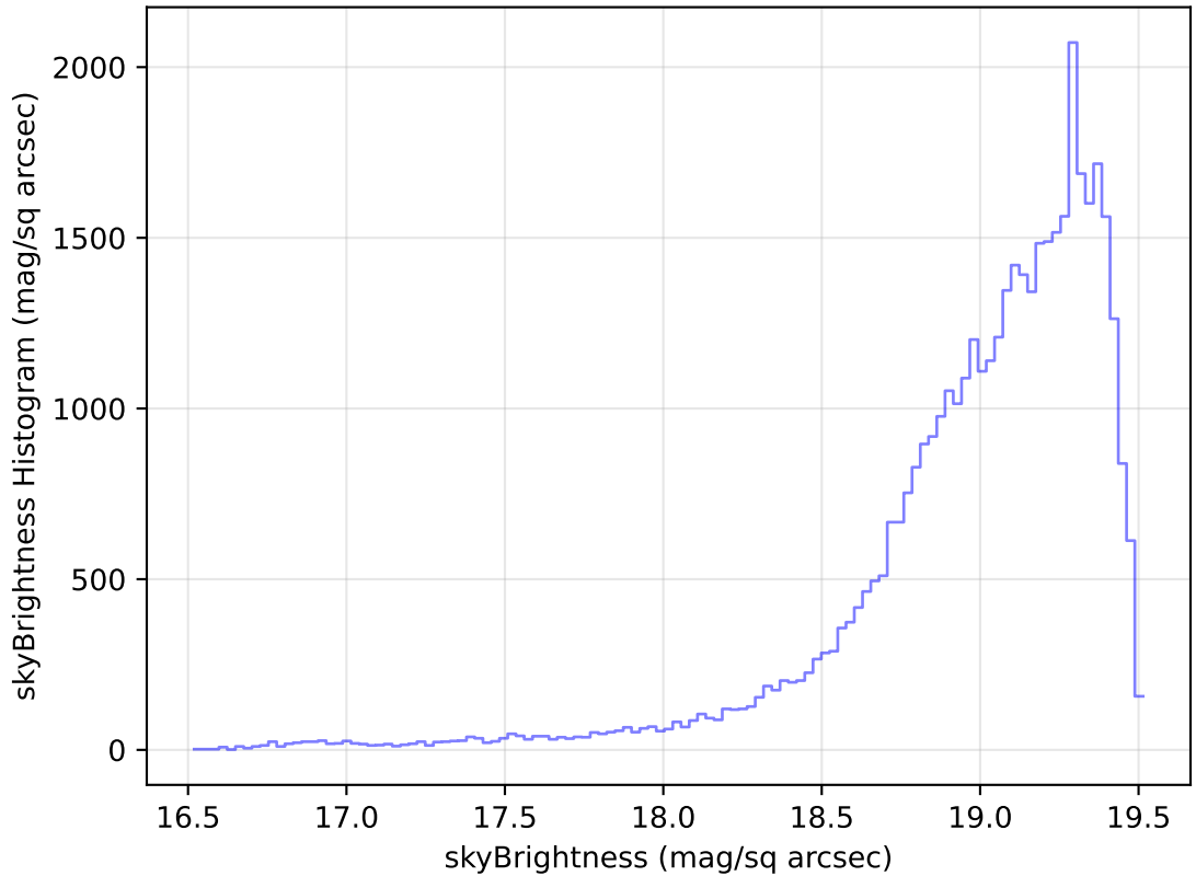
internal_u_expt38_nscale1.2v3.4_10yrs Yr 1 z band: skyBrightness Histogram
