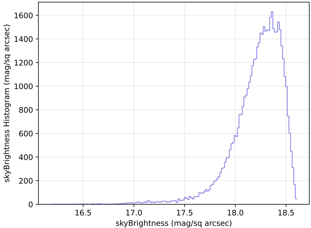
internal_u_expt38_nscale1.2v3.4_10yrs Yr 1 y band: skyBrightness Histogram
