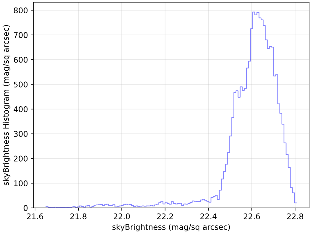
internal_u_expt38_nscale1.2v3.4_10yrs Yr 1 u band: skyBrightness Histogram
