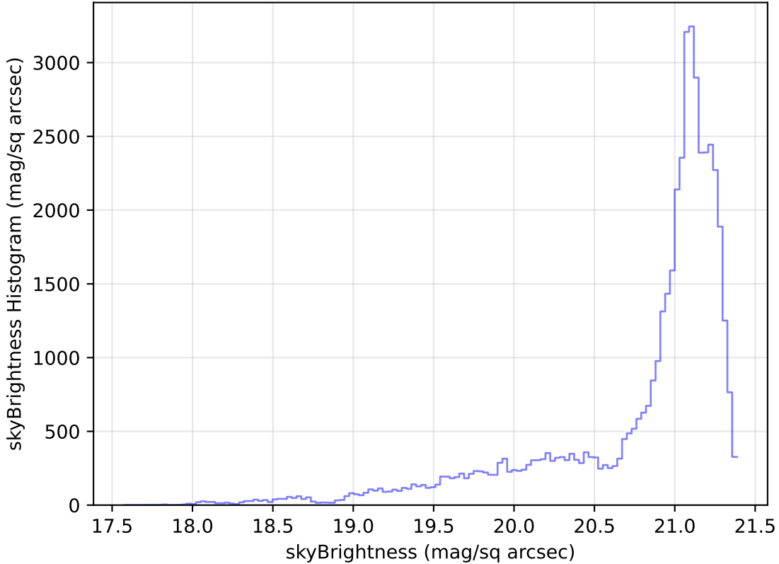
internal_u_expt38_nscale1.2v3.4_10yrs Yr 1 r band: skyBrightness Histogram
