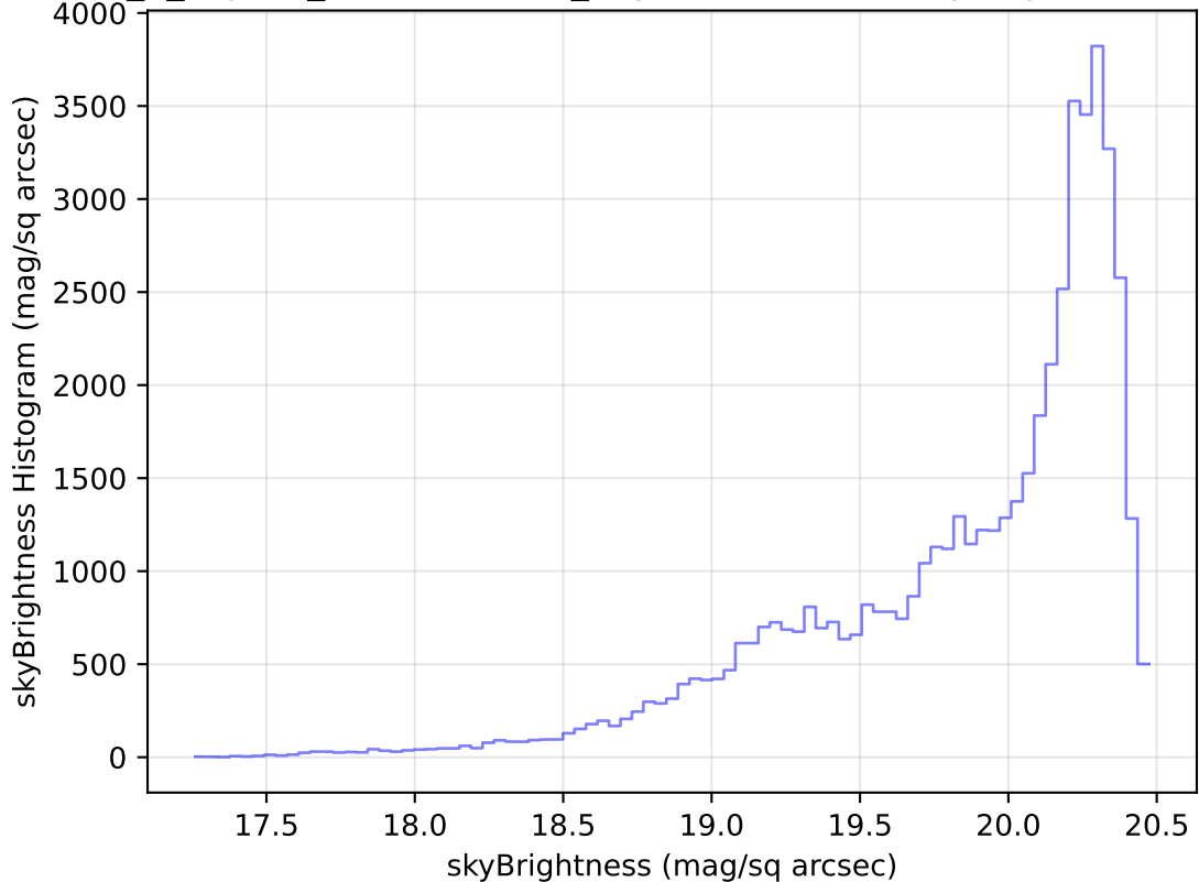
internal_u_expt38_nscale1.2v3.4_10yrs Yr 1 i band: skyBrightness Histogram
