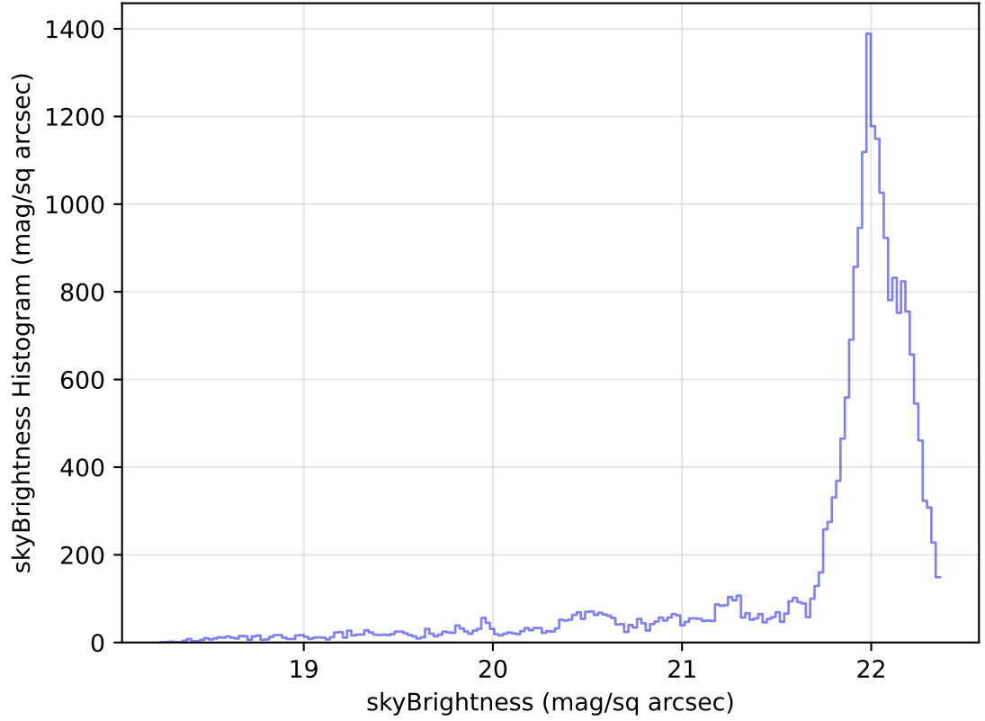
internal_u_expt38_nscale1.2v3.4_10yrs Yr 1 g band: skyBrightness Histogram
