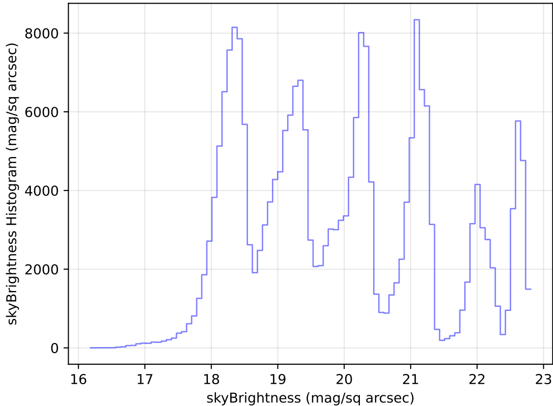
internal_u_expt38_nscale1.2v3.4_10yrs Yr 1 all bands: skyBrightness Histogram
