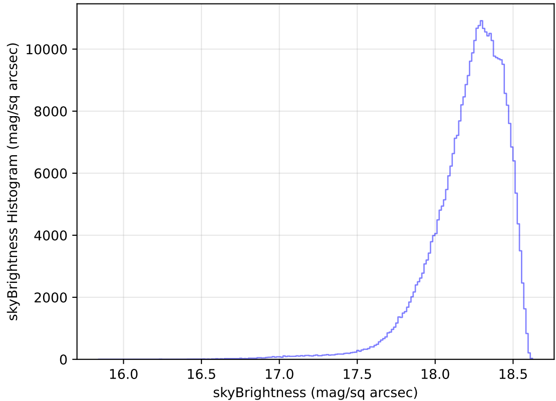
internal_u_expt38_nscale1.2v3.4_10yrs WFD y band: skyBrightness Histogram
