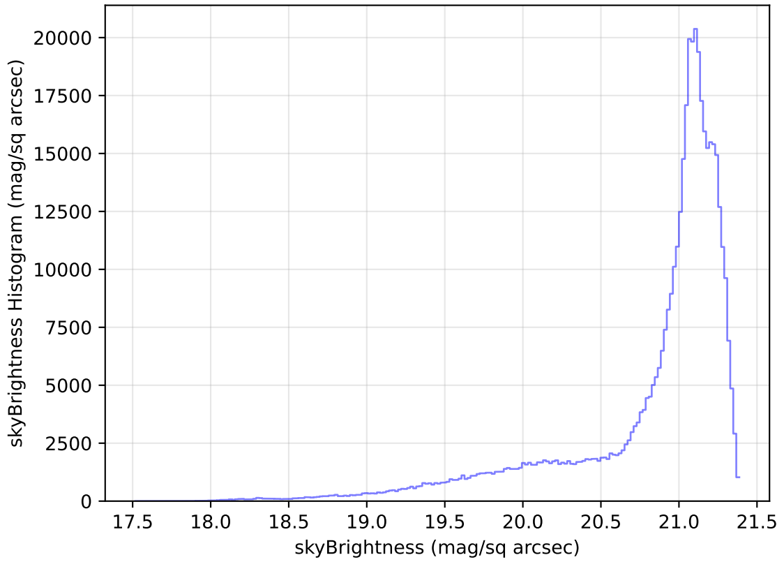
internal_u_expt38_nscale1.2v3.4_10yrs WFD r band: skyBrightness Histogram
