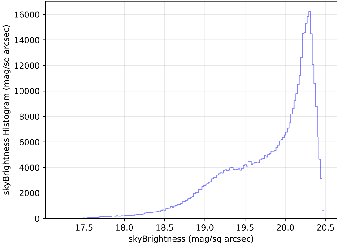
internal_u_expt38_nscale1.2v3.4_10yrs WFD i band: skyBrightness Histogram
