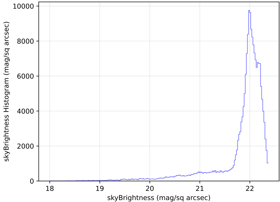
internal_u_expt38_nscale1.2v3.4_10yrs WFD g band: skyBrightness Histogram
