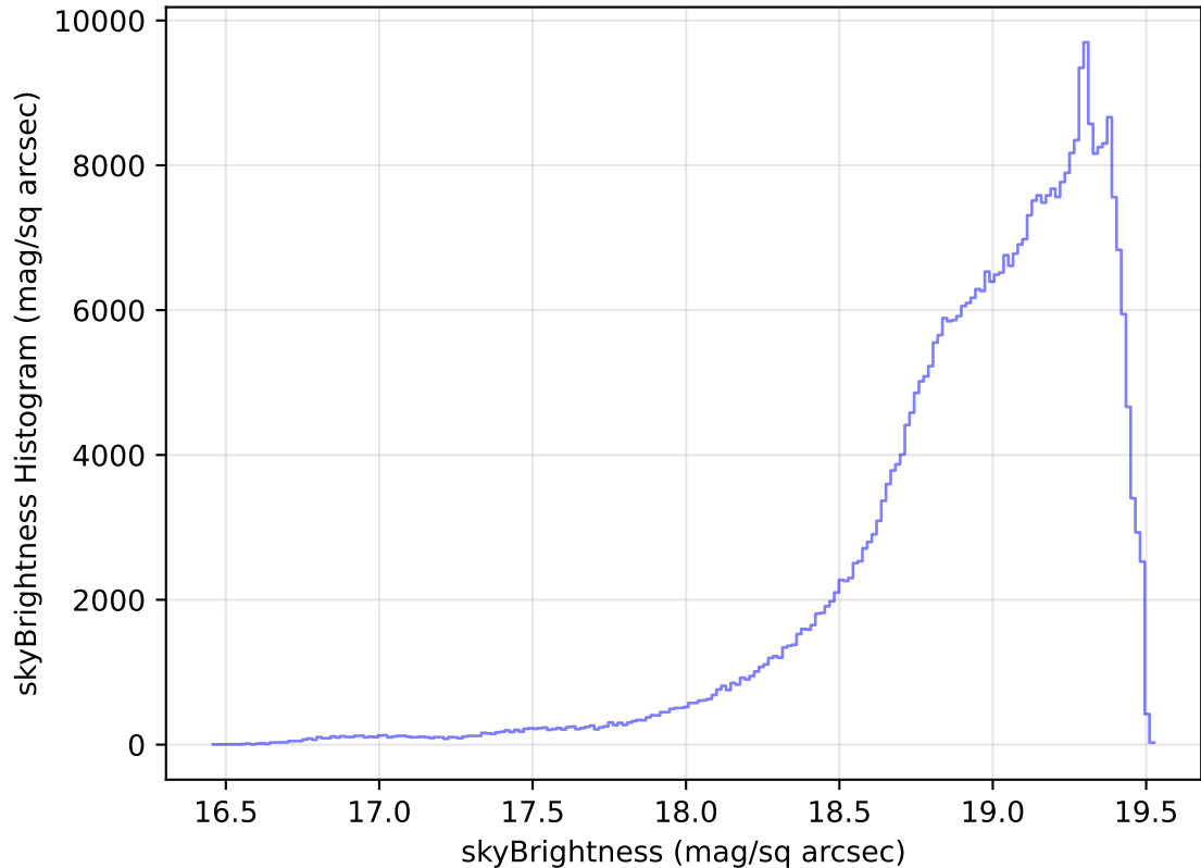
internal_u_expt38_nscale1.2v3.4_10yrs All sky z band: skyBrightness Histogram
