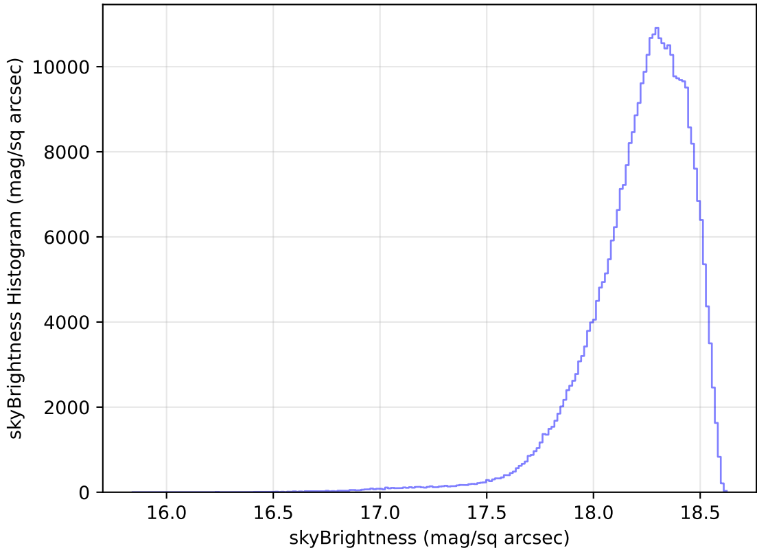
internal_u_expt38_nscale1.2v3.4_10yrs All sky y band: skyBrightness Histogram
