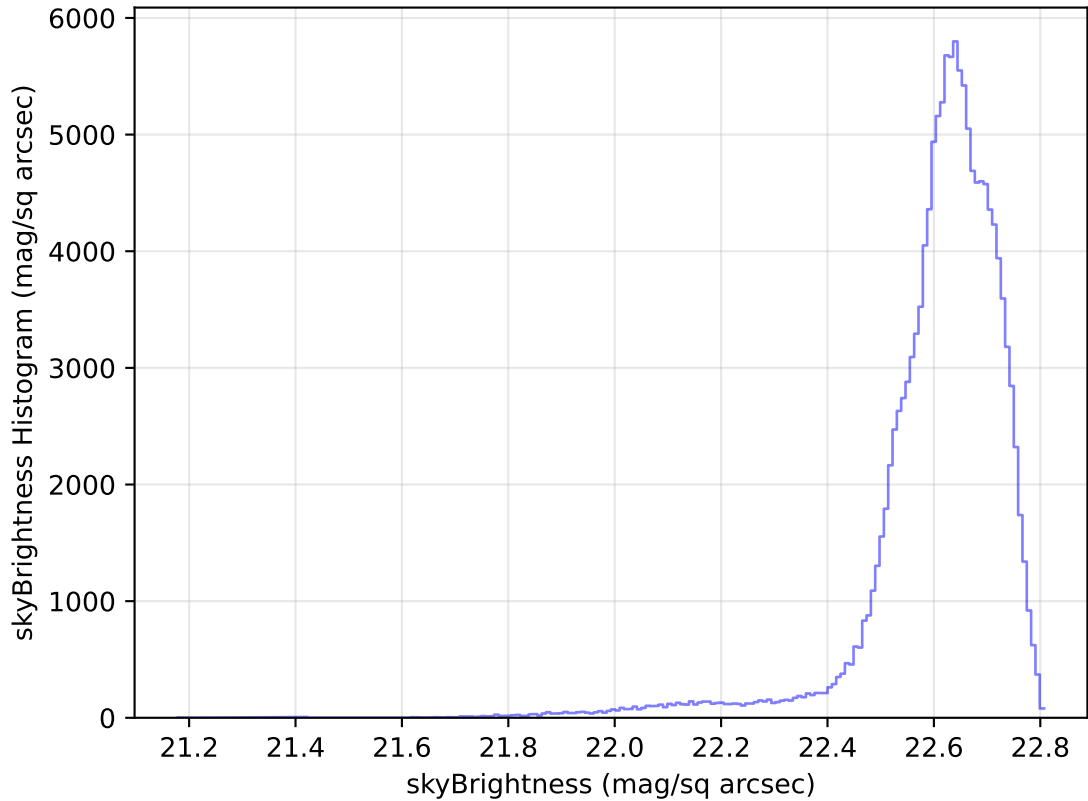
internal_u_expt38_nscale1.2v3.4_10yrs All sky u band: skyBrightness Histogram
