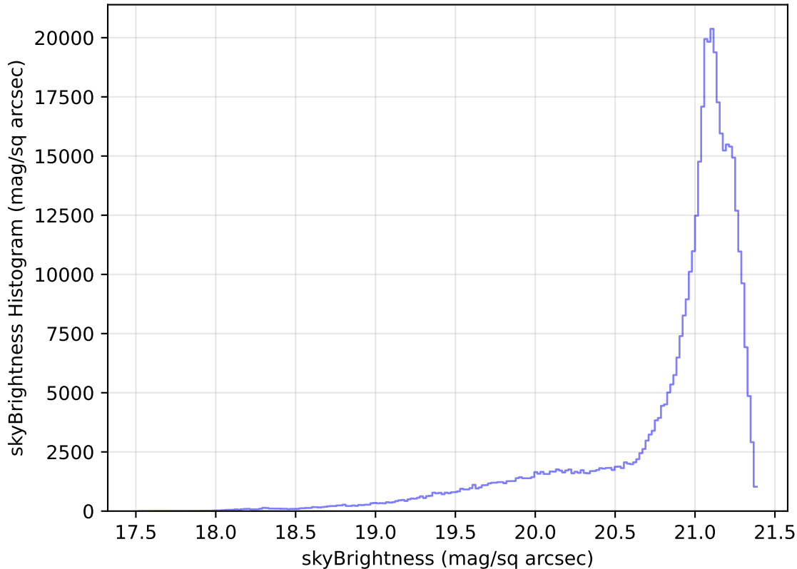
internal_u_expt38_nscale1.2v3.4_10yrs All sky r band: skyBrightness Histogram
