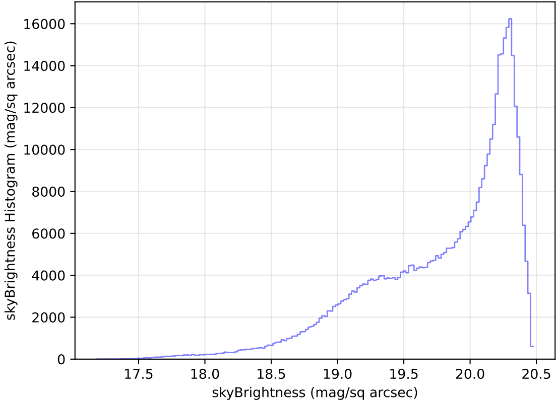
internal_u_expt38_nscale1.2v3.4_10yrs All sky i band: skyBrightness Histogram
