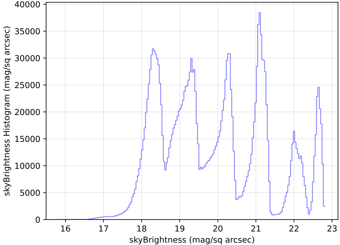
internal_u_expt38_nscale1.2v3.4_10yrs All sky all bands: skyBrightness Histogram
