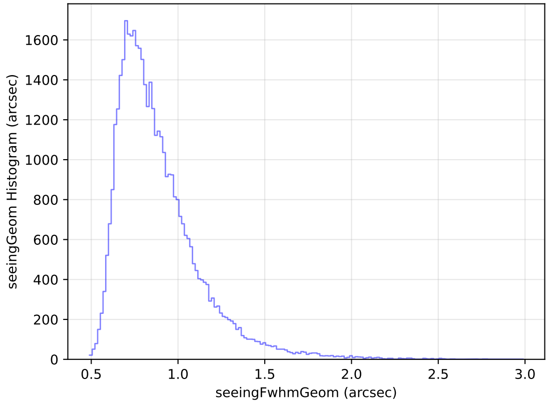
internal_u_expt38_nscale1.2v3.4_10yrs Yr 1 z band: seeingGeom Histogram
