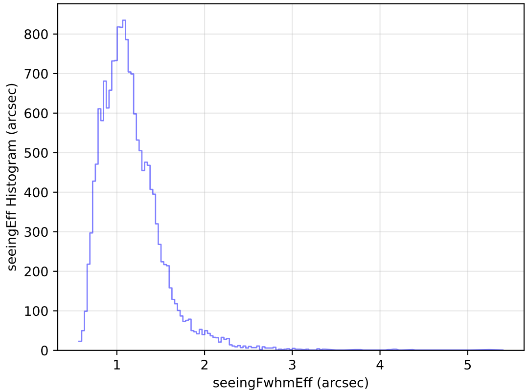
internal_u_expt38_nscale1.2v3.4_10yrs Yr 1 u band: seeingEff Histogram
