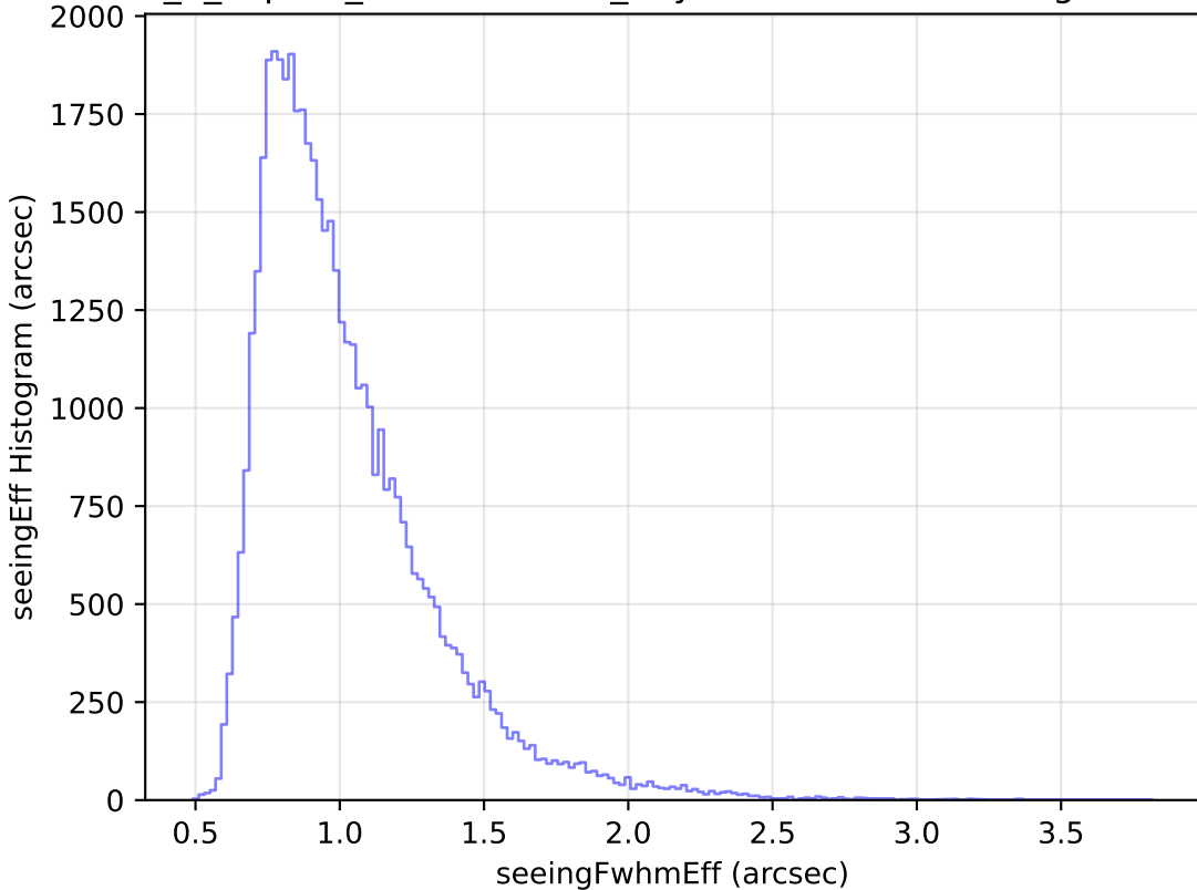
internal_u_expt38_nscale1.2v3.4_10yrs Yr 1 r band: seeingEff Histogram
