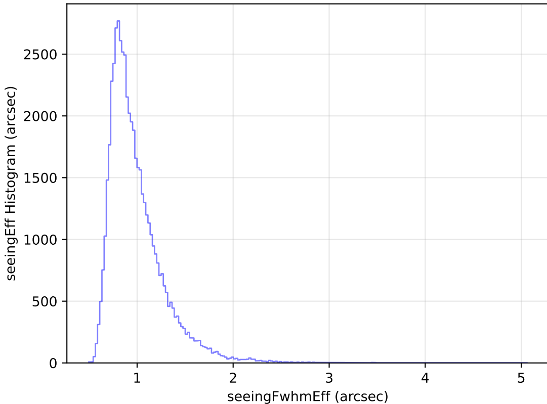
internal_u_expt38_nscale1.2v3.4_10yrs Yr 1 i band: seeingEff Histogram
