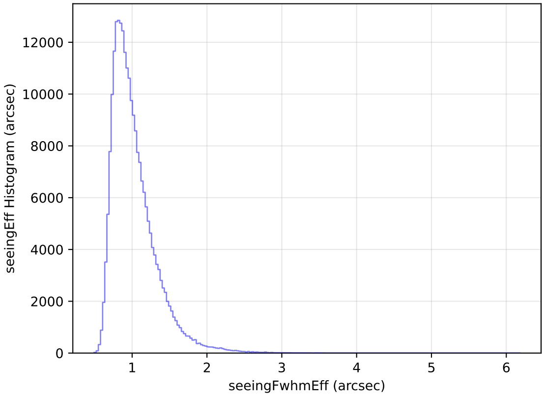
internal_u_expt38_nscale1.2v3.4_10yrs Yr 1 all bands: seeingEff Histogram
